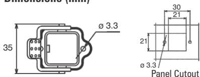
Dimensions (mm)
