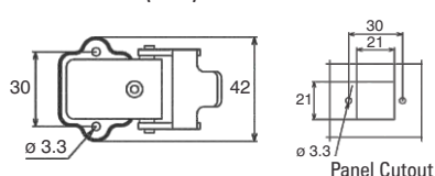
Dimensions (mm)
