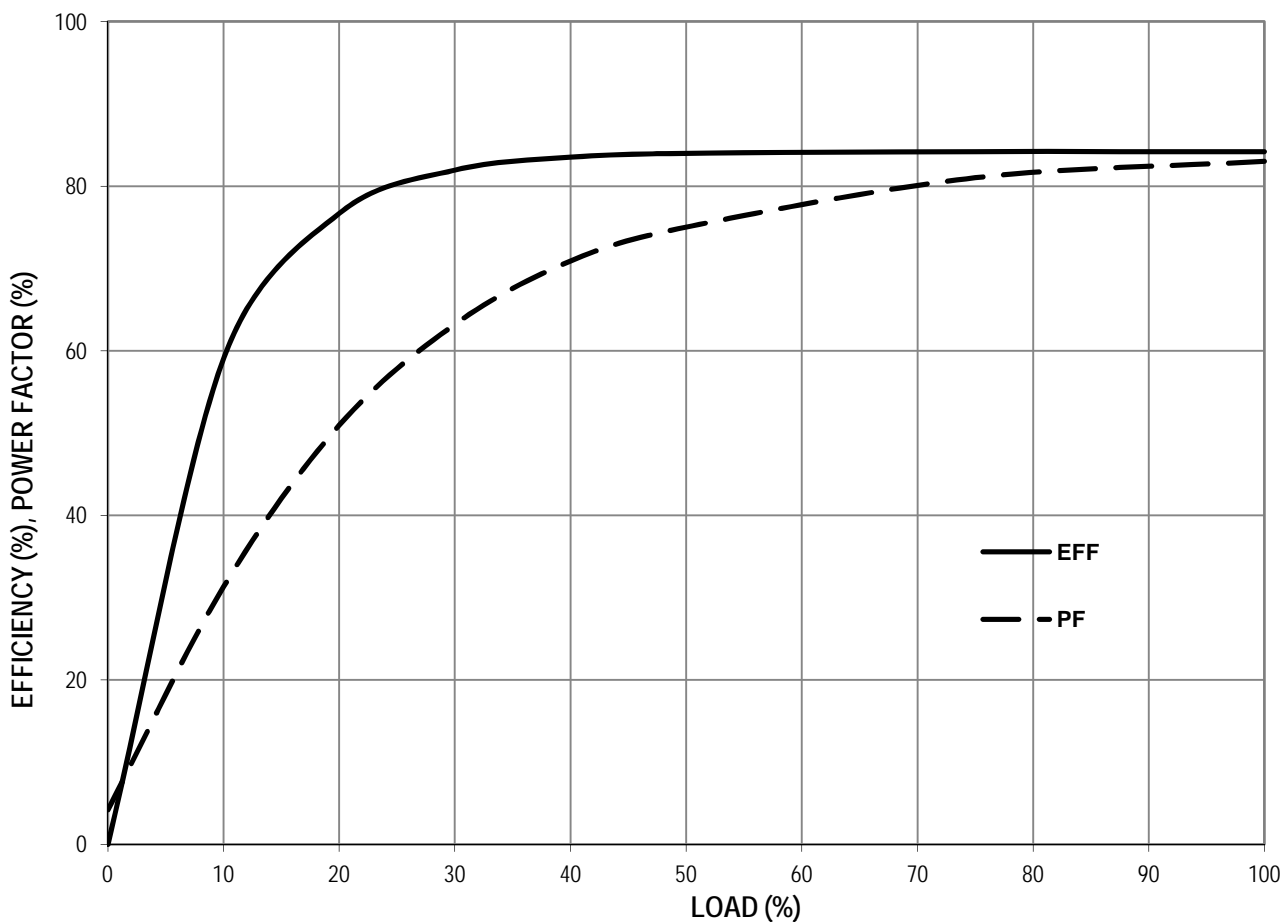
LOAD-EFFICIENCY-POWER FACTOR CURVE
