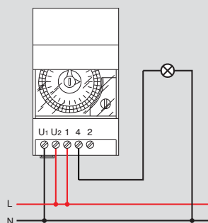
MicroRex – 3 modules
