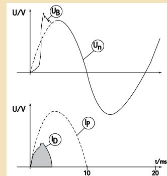
Current limiting DX 3 MCB
