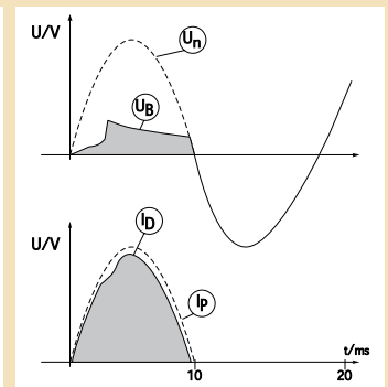
Zero point extinguishing MCB
