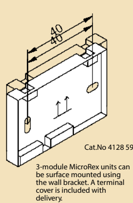
Wall bracket - 3 modules
